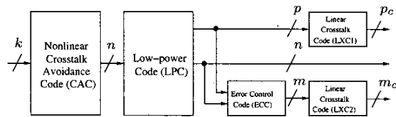
Figure 2: A unified coding framework.
