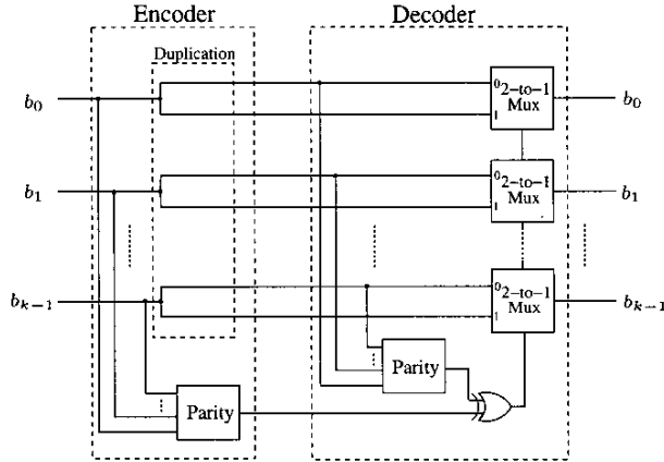
Figure 3: CAC+ECC: Duplicate-add-parity (DAP)
