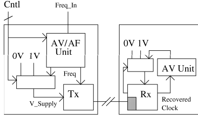
Figure 3: Block Diagram of a Link
