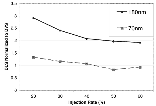
Figure 8: Energy Consumption with Technology Scaling
