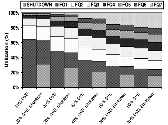
Figure 7: Frequency Profiling with Both DVS and DLS
