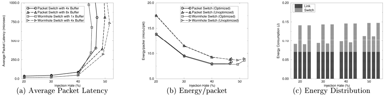
Figure 9: 8x8 Mesh Network Results (70nm design)
