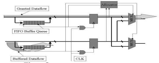
Figure 3: Buffers in a 2 \times 2 Node Switch
