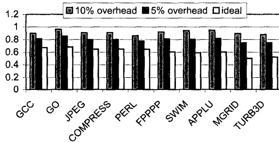
Figure 12. Normalized EPI for an 8-stage pipeline (200k trace-cache)
