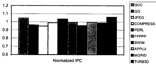
Figure 8. IPC variation for the 14-stage pipelines (100k trace-cache)
