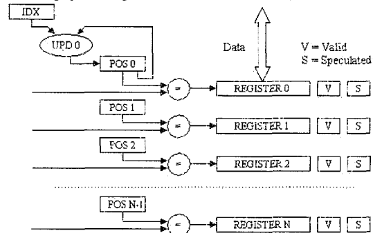
Figure 3. Architected register structure
