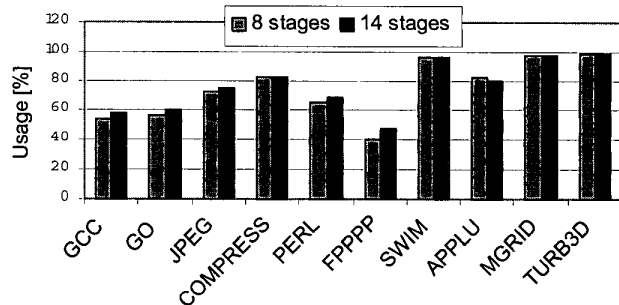
Figure 10. Alternative execution path usage (100k trace-cache)
