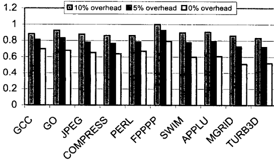
Figure 7. Normalized EPI for an 8-stage pipeline (100k trace-cache)
