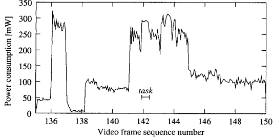
Figure 7: Processor power consumption of EPS.
