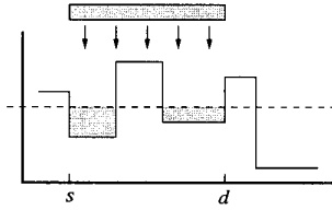
Figure 3: Task leveling.
