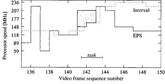
Figure 6: Clock schedules executed by PowerScale.
