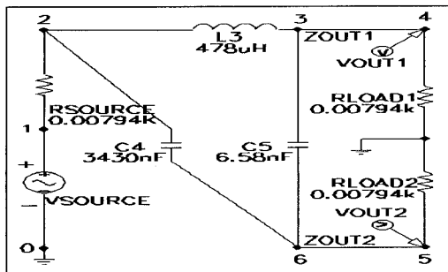
Figure 8 Best circuit of generation 0.
