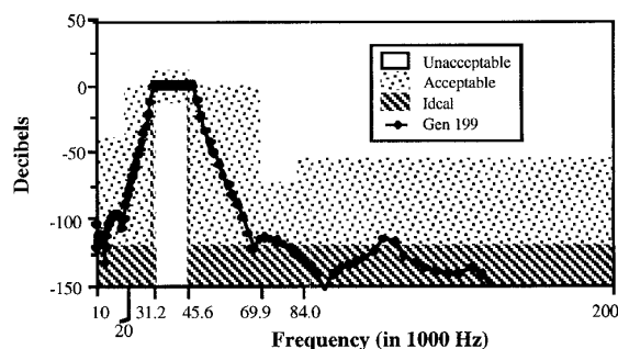
Figure 21 Frequency domain behavior of best-of-run circuit of generation 199.
