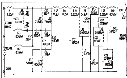
Figure 20 Best-of-run circuit of generation 199.
