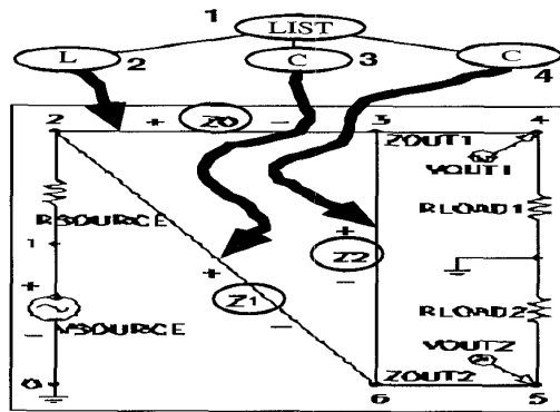
Figure 1 One-input, two-output embryonic electrical circuit.
