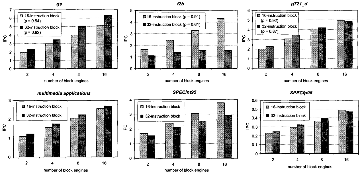
Figure 9. IPC as a function of the number of block engines and BSA-block size. Perfect caches were assumed in these experiments.
