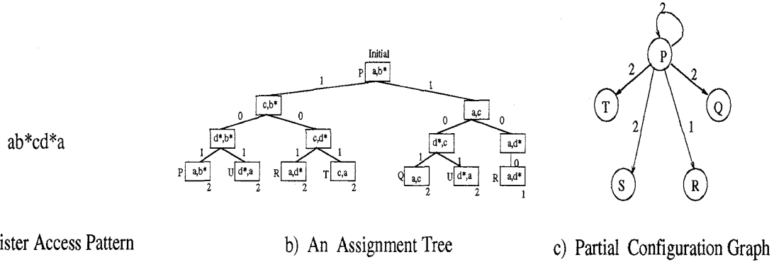
Figure 3: Building a configuration graph from the assignment trees.
